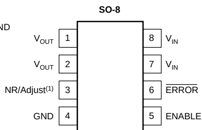
(U Package)
