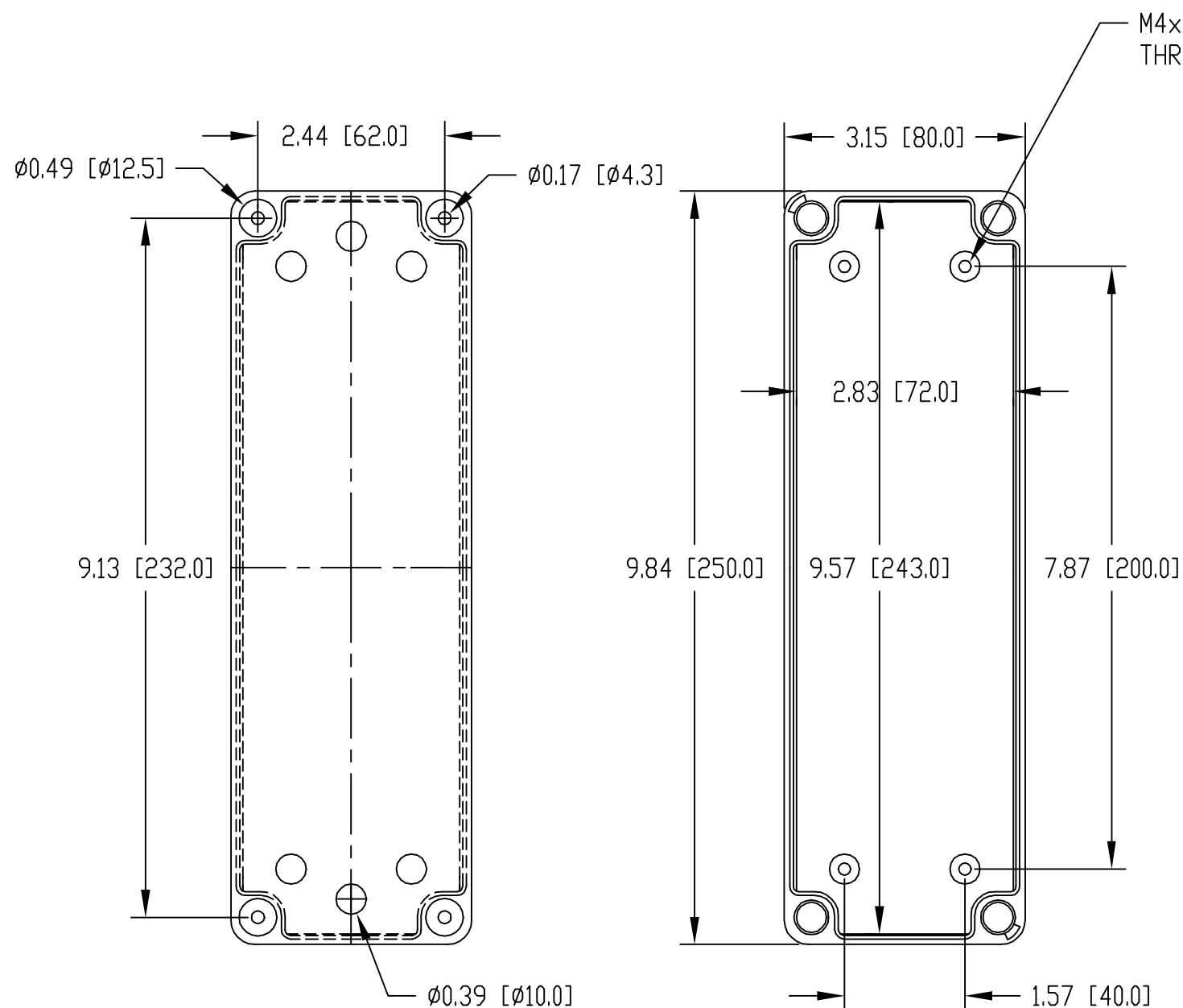
BOTTOM VIEW
