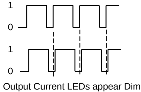
PWM Digital Control Signal
