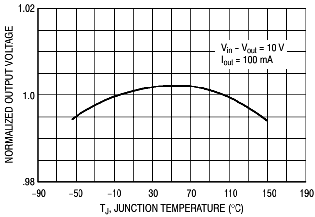
Figure 4. Temperature Stability
