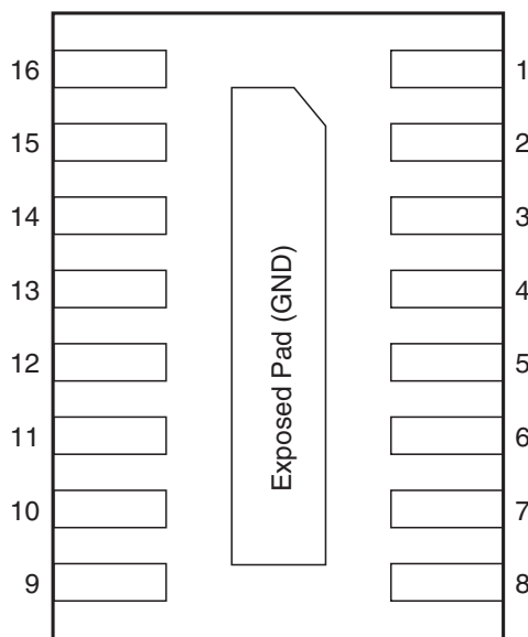
TDFN-16/DFN-16 (Bottom View)
