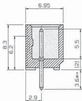
SECT. G-G
