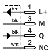
M8, 4-pin
