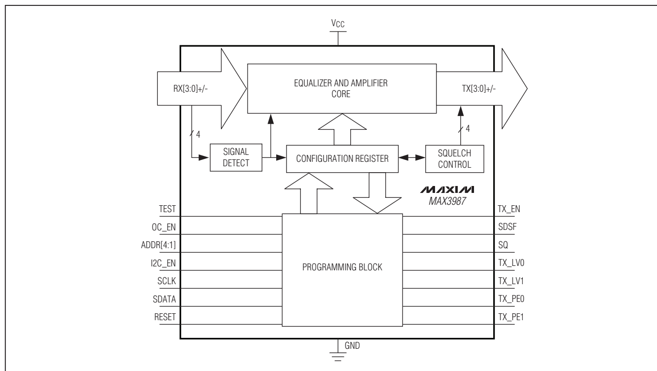
Figure 5. Functional Diagram
