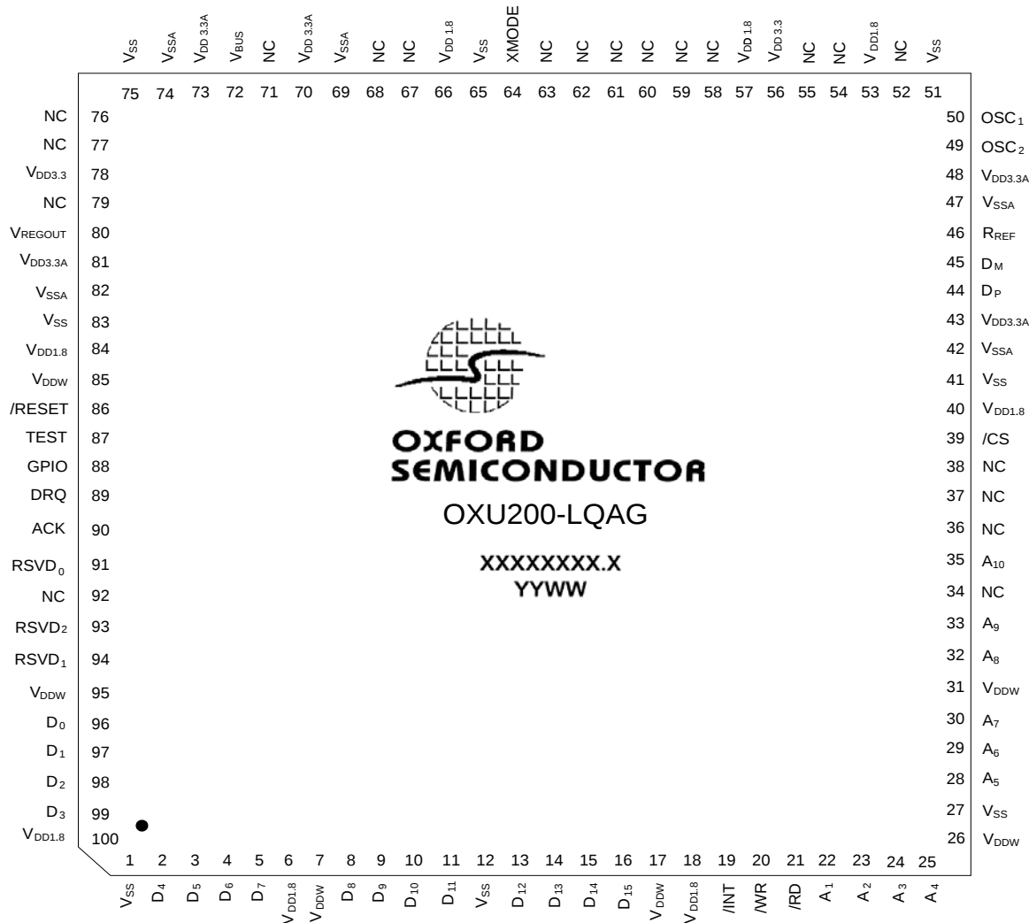
Figure 2 OXU200 100-Pin LQFP Package (Top View)
