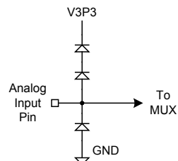
Analog Input Equivalent Circuit
