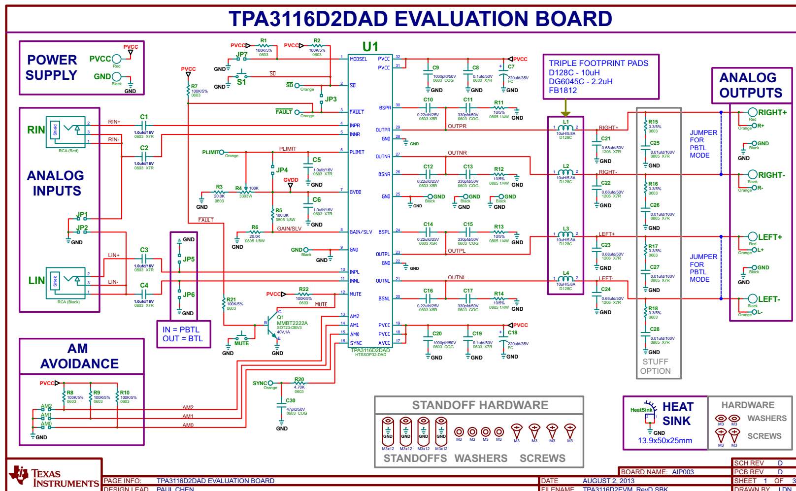
Figure 2. TPA3116D2EVM Schematic
