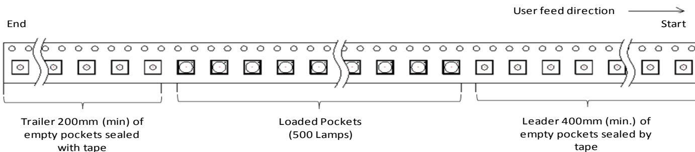
Tape Drawing
