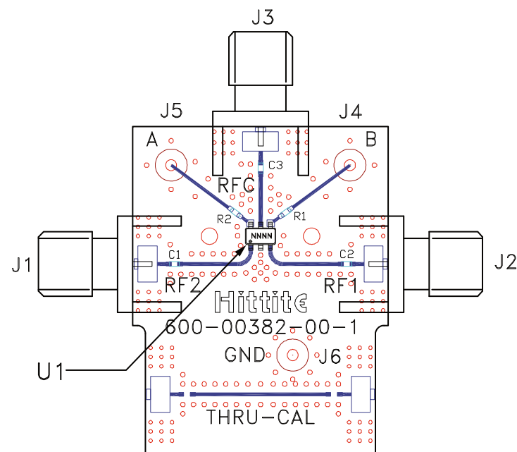
Figure 14. Evaluation PCB
