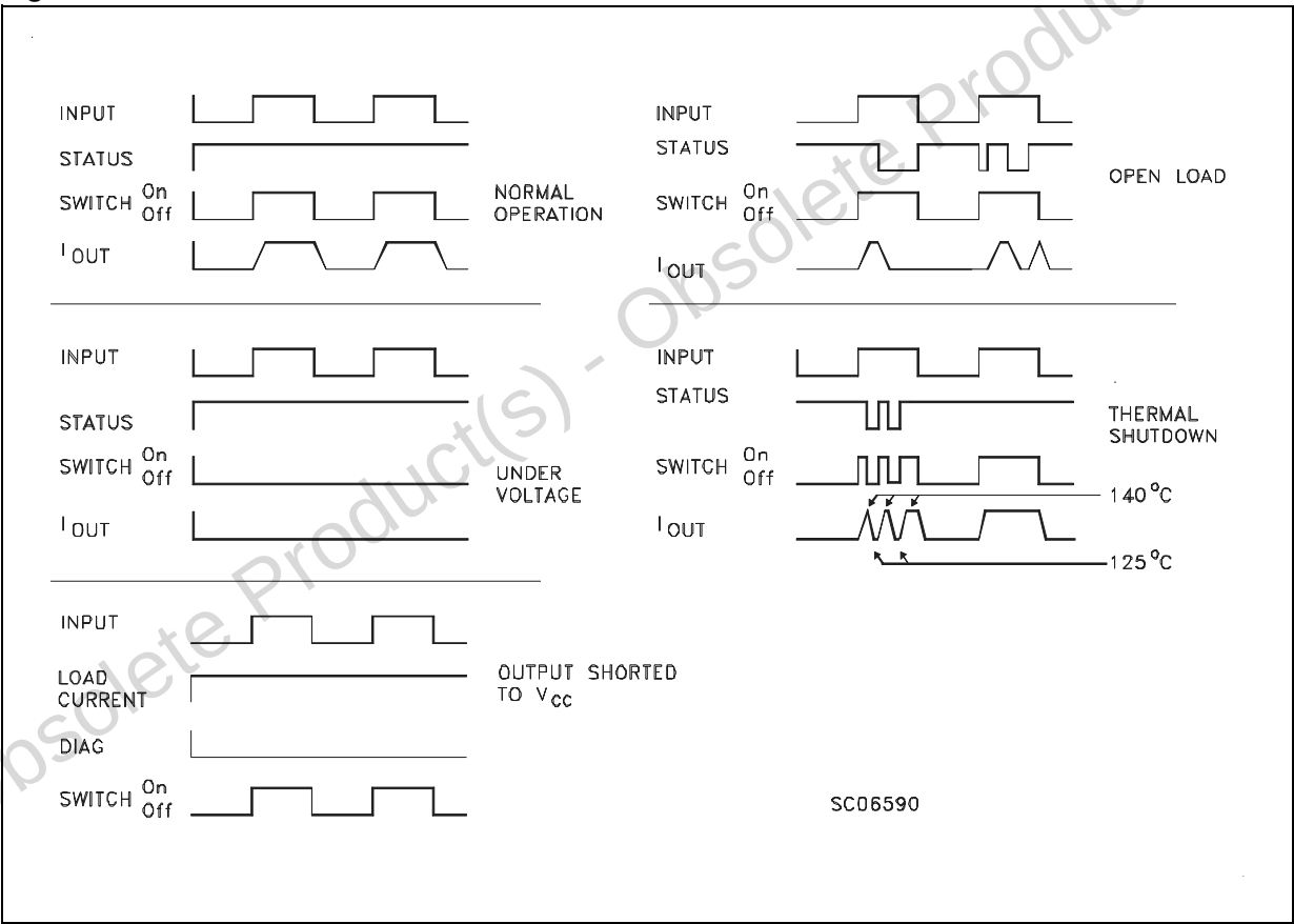
Figure 8. Waveforms
