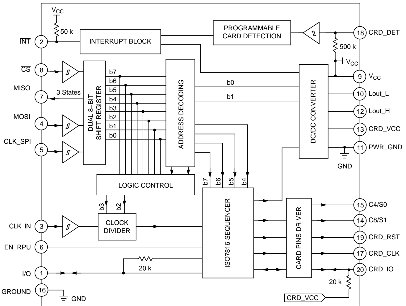
Figure 2. Block Diagram
