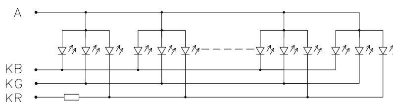
CIRCUIT DIAGRAM
