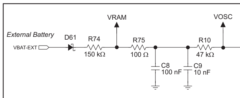
Figure D-2. RCM3309/RCM3319 Backup Battery Circuit
