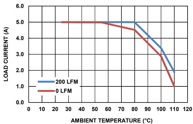
FIGURE 33. DERATING CURVES AT VIN = 3.3V, VOUT = 2.5V
