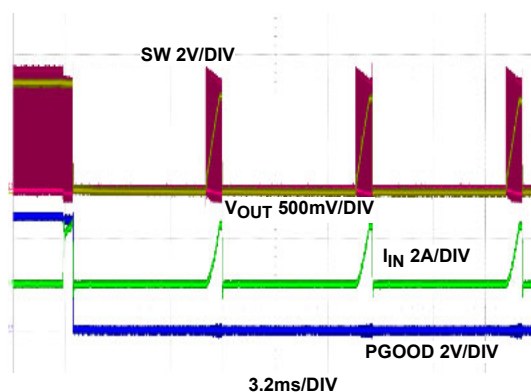
FIGURE 25. OUTPUT SHORT-CIRCUIT PROTECTION, HICCUP MODE
