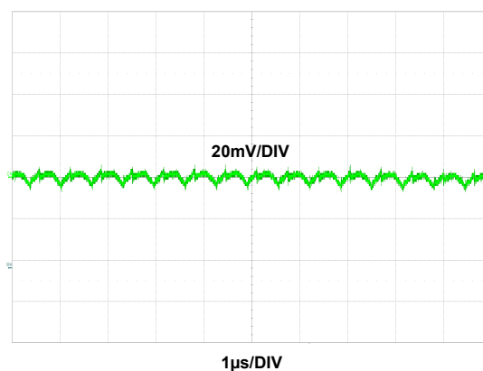
FIGURE 11. V_{IN} = 5V , V_{OUT} = 1.2V , I_{OUT} = 5A , f_{SW} = 1.6MHz , C_{OUT} = 2 \times 22\mu F CERAMIC CAPACITORS
