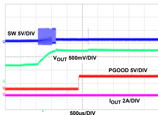
FIGURE 23. PREBIAS SOFT-START WITH 0A LOAD PFM MODE, V_{IN} = 5V , V_{OUT} = 1.2V , I_{OUT} = 0A , C_{OUT} = 2 \times 22\mu F CERAMIC CAPACITORS, C_{IN} = 100\mu F POSCAP + 2 \times 22\mu F CERAMIC CAPACITORS
