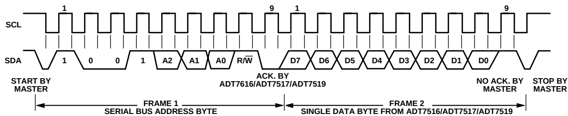
Figure 62. I²C—Reading a Single Byte of Data from a Selected Register
