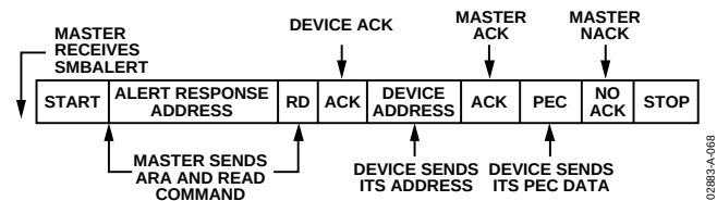
Figure 69. INT/ \overline{\text{INT}} Responds to \overline{\text{SMBALERT}} ARA with Packet Error Checking (PEC)
