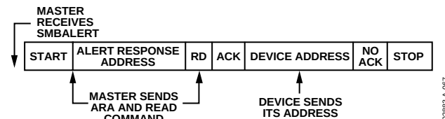
Figure 68. INT/ \overline{\text{INT}} Responds to \overline{\text{SMBALERT}} ARA
