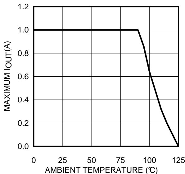
Figure 23. Thermal Derating Curve
