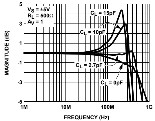
FIGURE 6. FREQUENCY RESPONSE vs C_L
