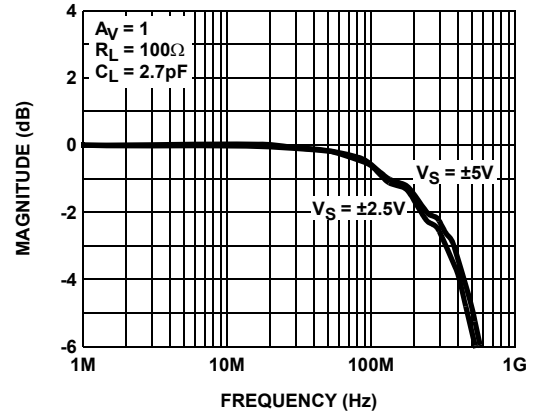
FIGURE 4. FREQUENCY RESPONSE vs SUPPLY VOLTAGE
