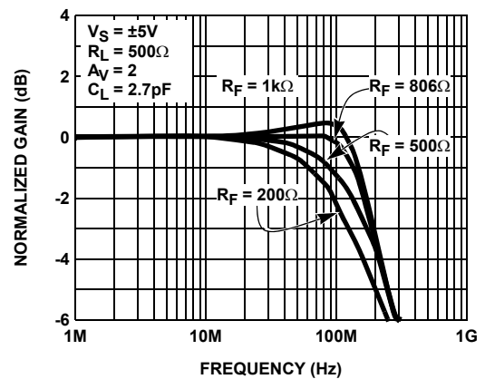
FIGURE 8. FREQUENCY RESPONSE FOR VARIOUS R_F
