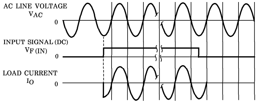
Fig.1 SWITCHING WAVEFORM
