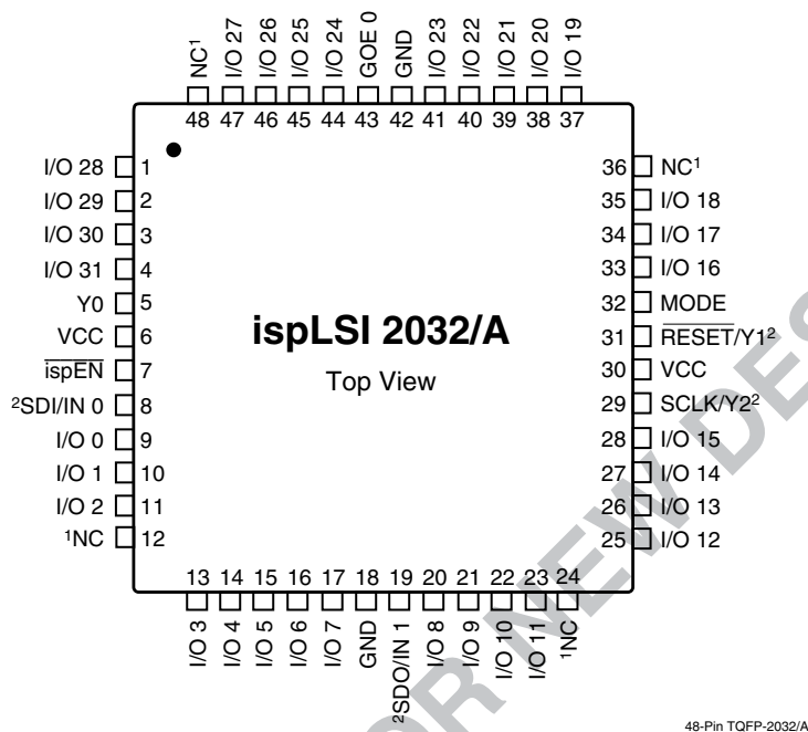
ispLSI 2032/A 48-Pin TQFP Pinout Diagram
