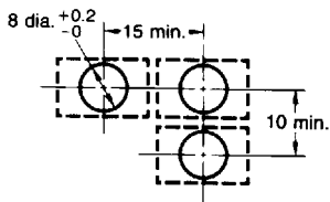
Panel cutout
