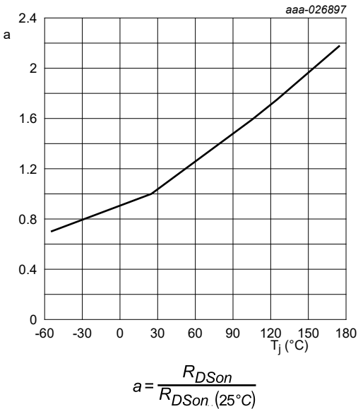
Fig. 11. Normalized drain-source on-state resistance factor as a function of junction temperature, FET1 and FET2
