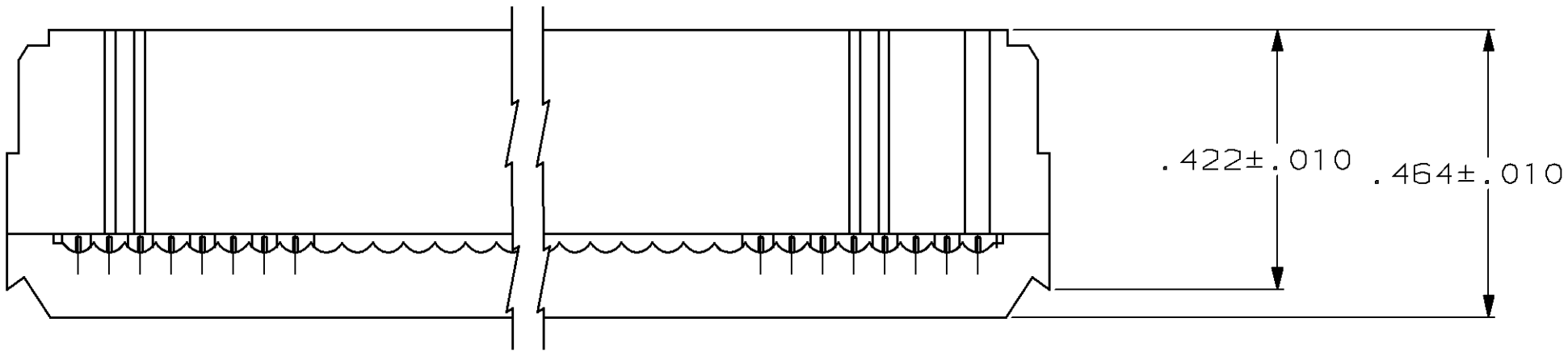
TERMINATED VIEW
