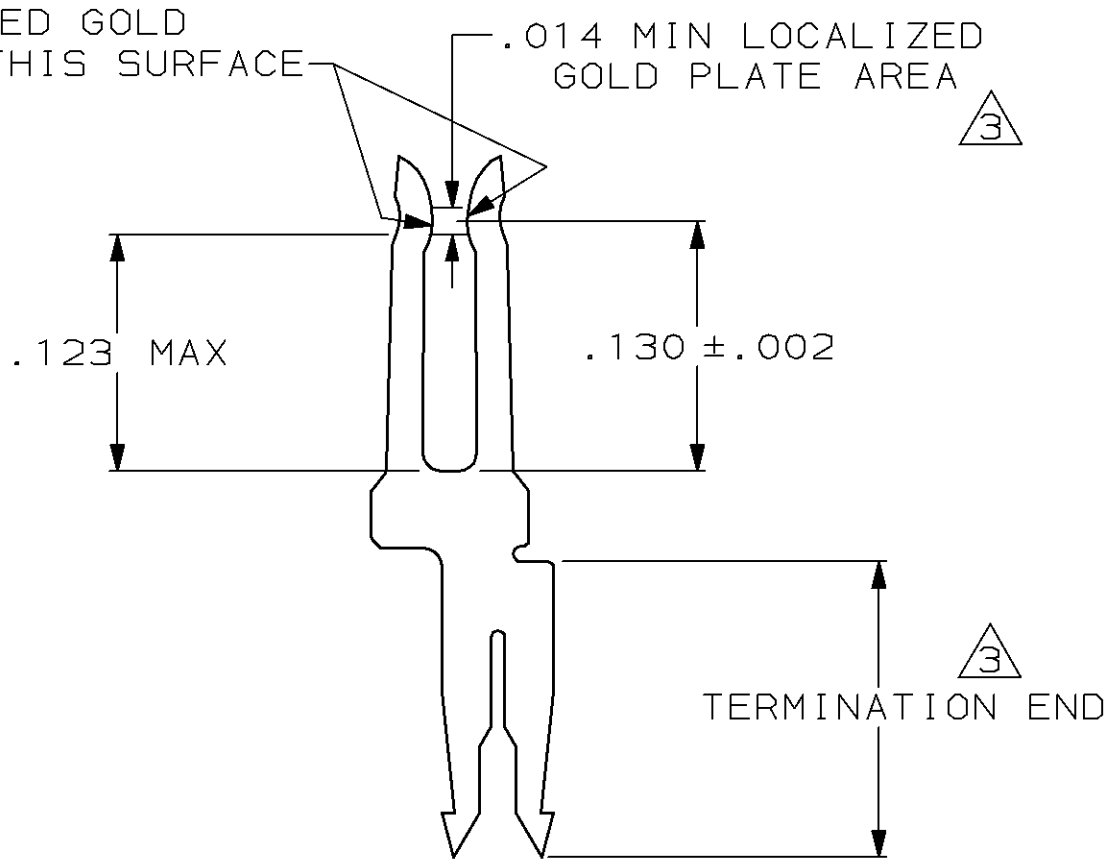
DETAIL Z SCALE 10:1 TYPICAL
