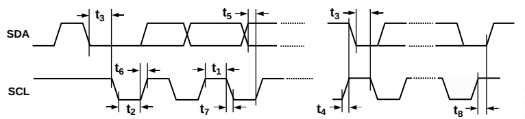
Figure 19. MPU Port Timing Diagram ( \text{I}^2\text{C} Mode)
