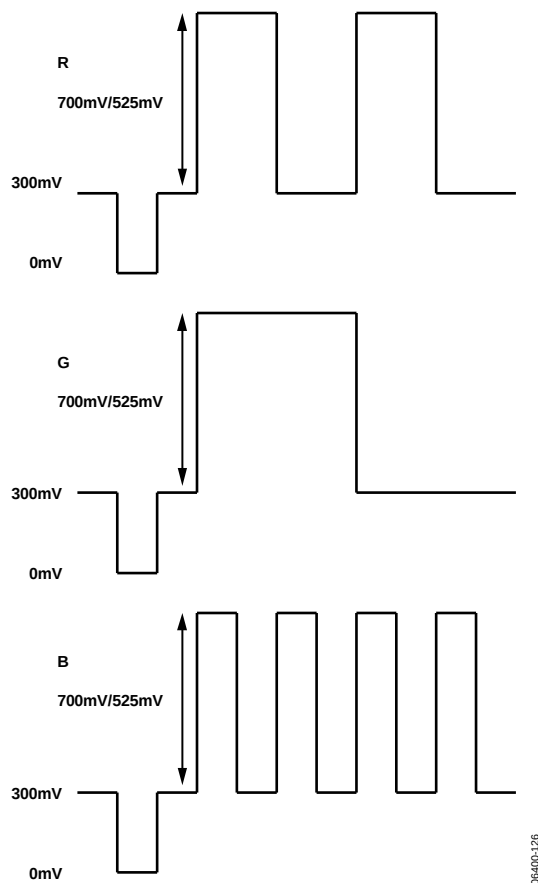
Figure 123. SD/ED RGB Output Levels—RGB Sync Enabled
