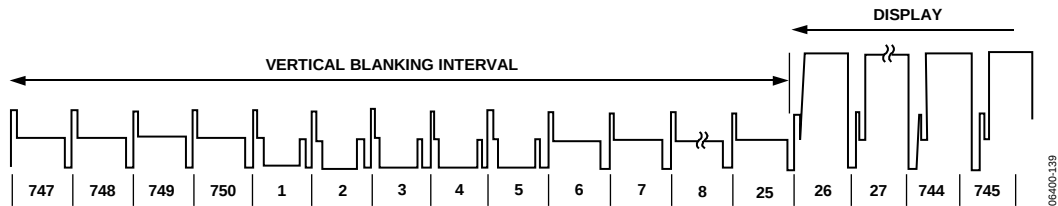
Figure 136. SMPTE 296M (720p)
