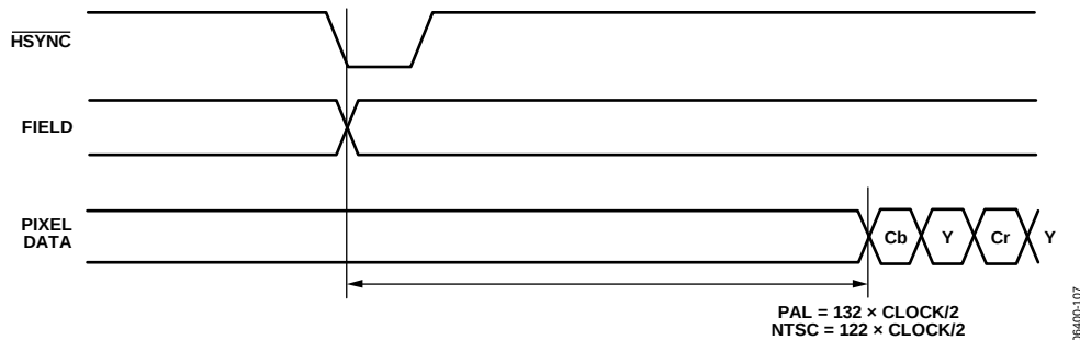
Figure 104. SD Timing Mode 1, Odd/Even Field Transitions (Master/Slave)
