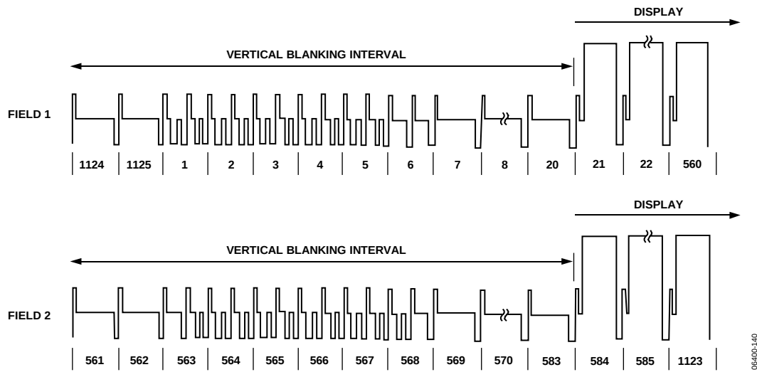
Figure 137. SMPTE 274M (1080i)
