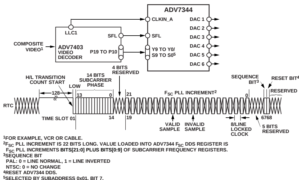
Figure 58. SD Subcarrier Frequency Lock Timing and Connections Diagram (Subaddress 0x84, Bits[2:1] = 11)
