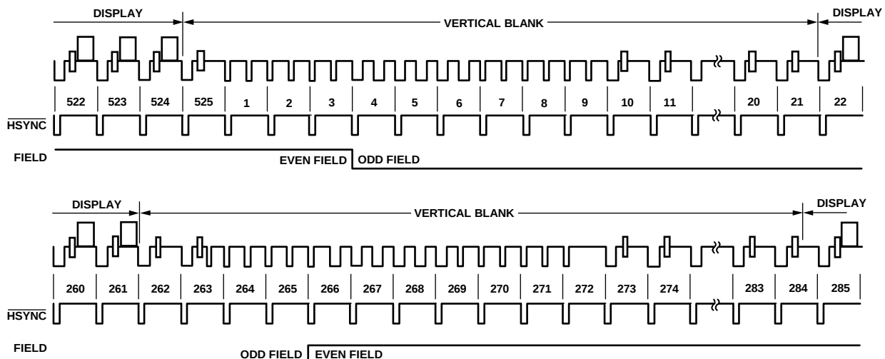
Figure 102. SD Slave Mode 1, NTSC
