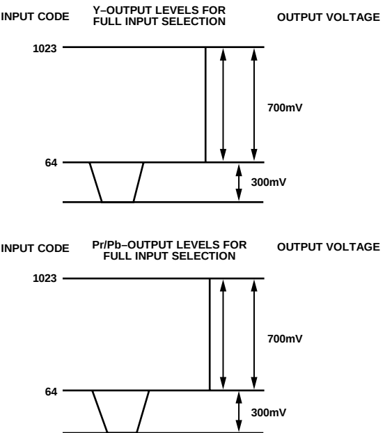
Figure 121. Output Levels for Full Input Selection
