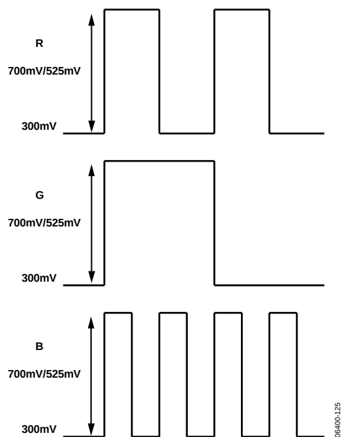
Figure 122. SD/ED RGB Output Levels—RGB Sync Disabled
