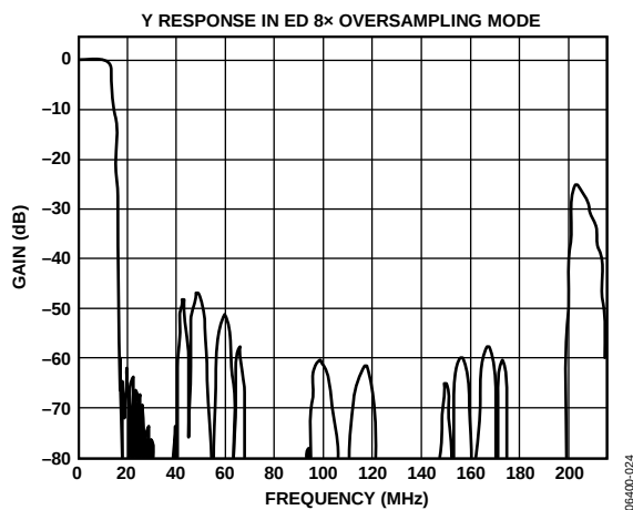
Figure 23. ED 8× Oversampling, Y Filter Response
