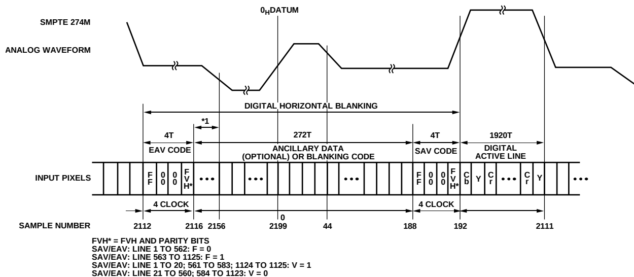
Figure 132. EAV/SAV Input Data Timing Diagram (SMPTE 274M)
