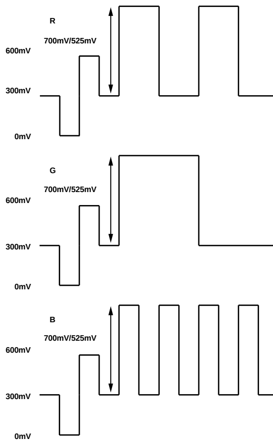
Figure 125. HD RGB Output Levels—RGB Sync Enabled
