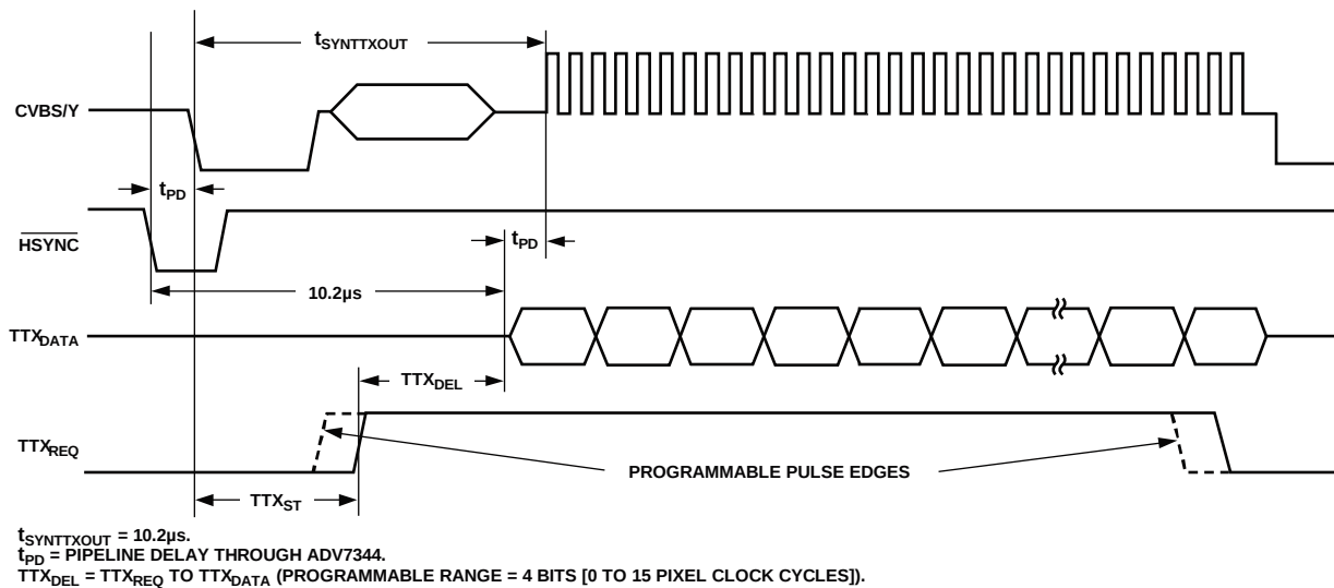
Figure 81. Teletext Functionality Diagram
