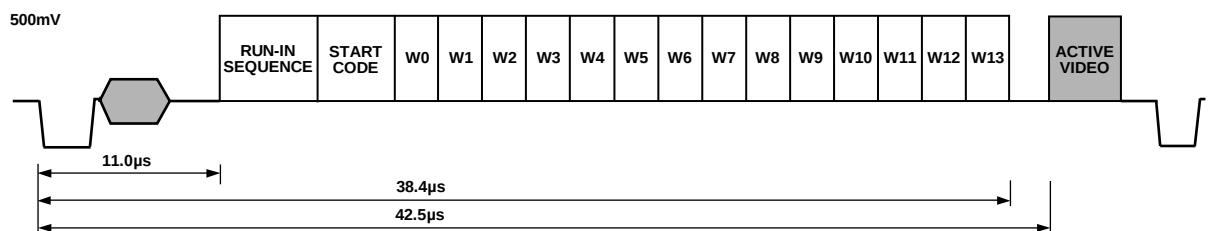
Figure 96. WSS Waveform Diagram
