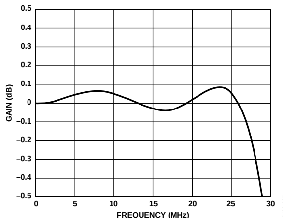
Figure 62. ED/HD Sinc Compensation Filter Enabled
