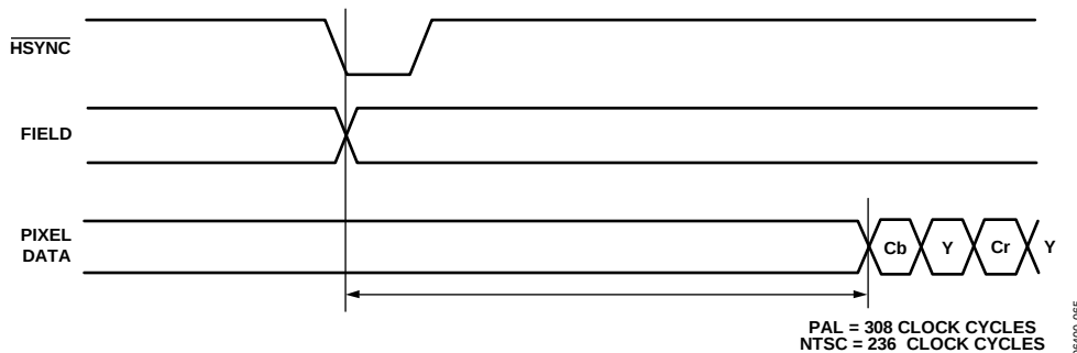
Figure 60. Square Pixel Mode Active Pixel Timing
