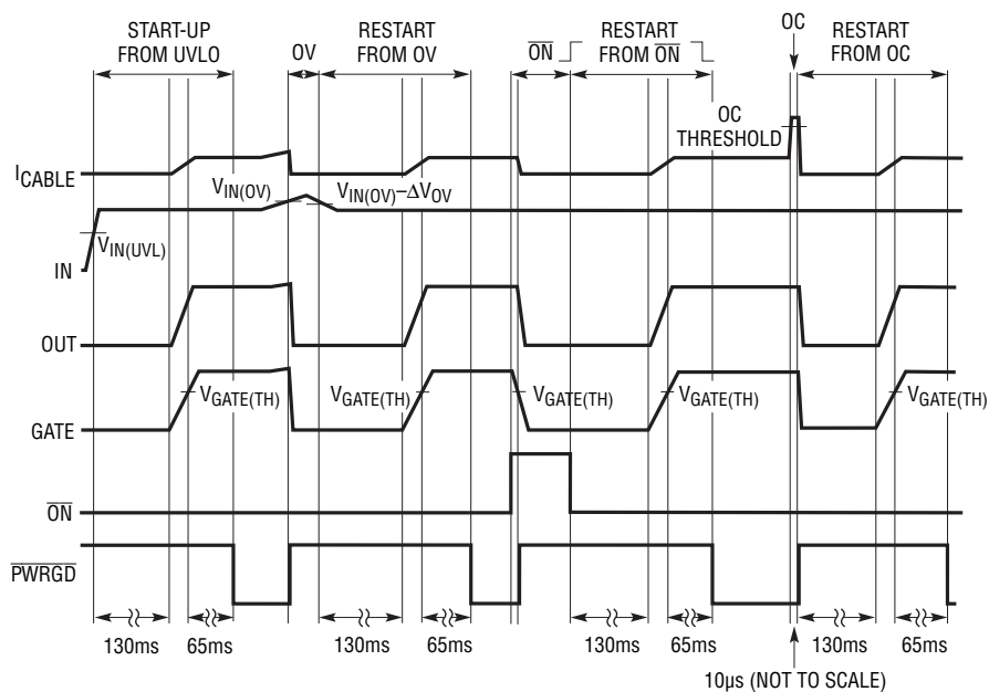
Figure 2. \overline{PWRGD} Behavior
