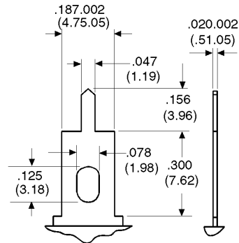
Printed Circuit Terminal
