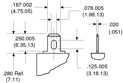
Solder/Plug In .187 Quick Connect
