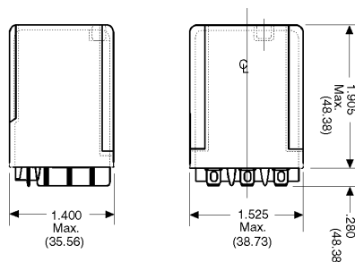
Dust Cover Model 157-2
