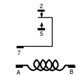
1 Form C (SPDT)
