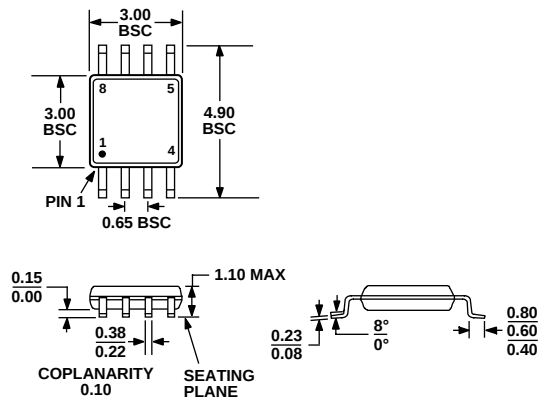
Figure 38. 8-Lead Mini Small Outline Package [MSOP] (RM-8)
