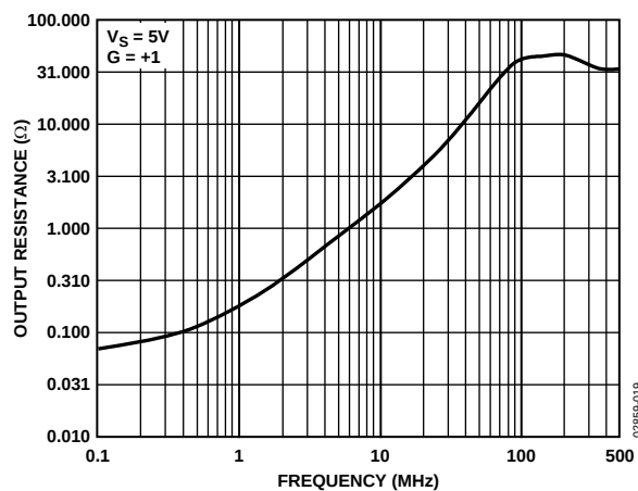
Figure 19. Closed-Loop Output Resistance vs. Frequency
