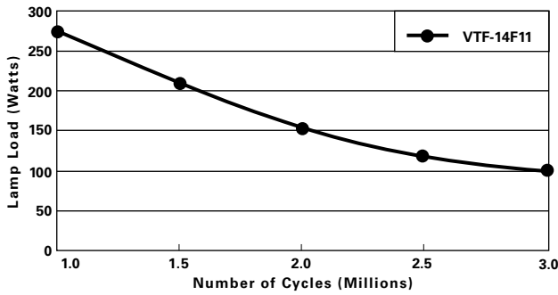
Figure 1 - Electrical Contact Life vs. Load Power
