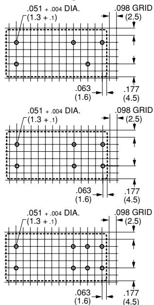
2 Form A, Standard Contact Gap
