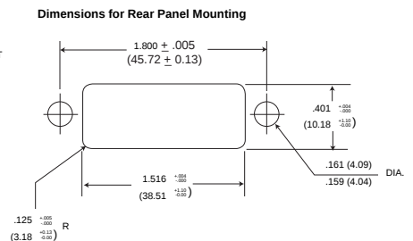
Dimensions for Rear Panel Mounting
