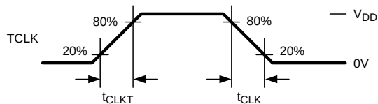
Figure 5. Serializer Input Clock Transition Times
