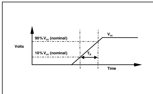
Figure 3.1 Ramp Rate Requirement
