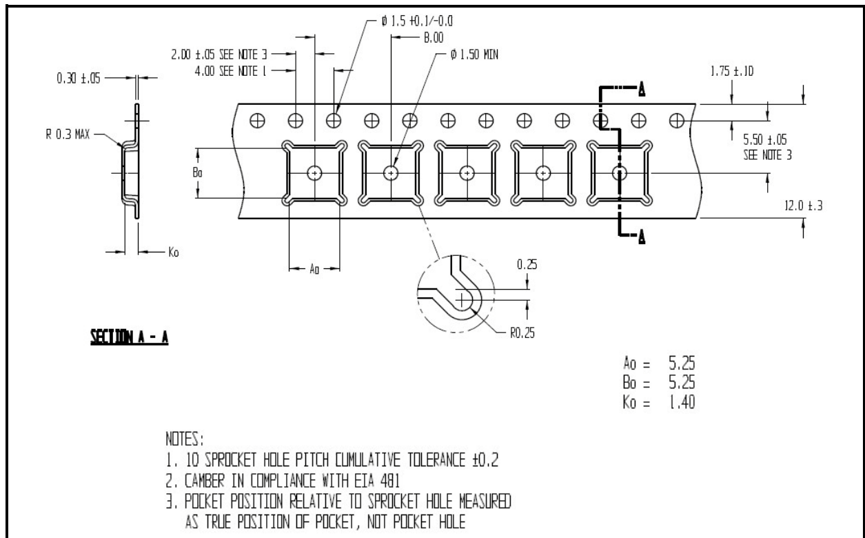
Figure 8: Detailed Tape and Reel Information (All dimensions in Millimeters)
