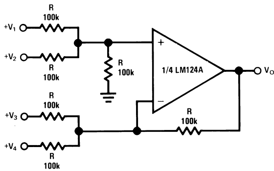
DC Summing Amplifier ( V_{\text{IN'S}} \geq 0\text{ V}_{\text{DC}} and V_O \geq V_{\text{DC}} )
