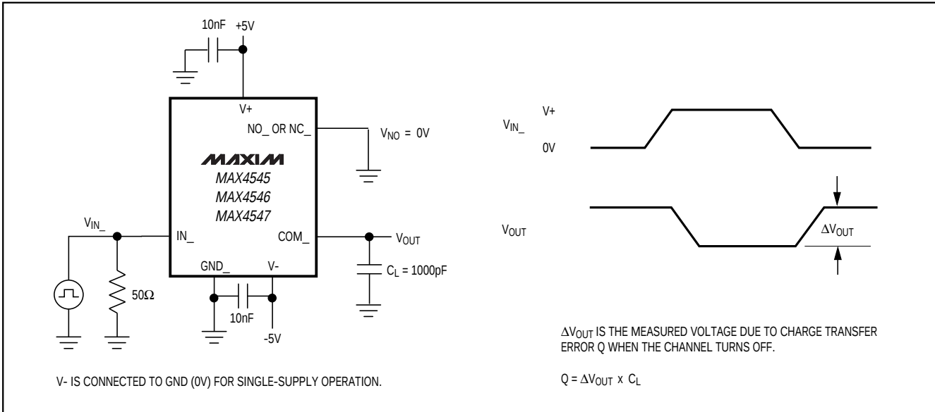
Figure 6. Charge Injection
