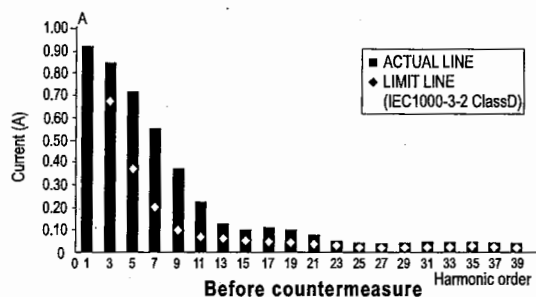
Characteristic of harmonic corrector (Test conditions: V_{in}=230VAC , W_{in}=200W , T_a=25^{\circ}C )
