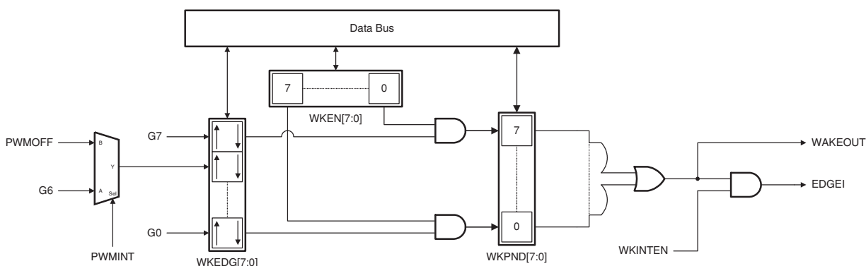
Figure 15. Multi-input Wakeup (MIW) Block Diagram 6
