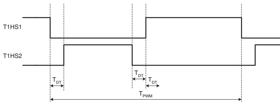
Figure 12. Example PWM Output Signals a) and b)
