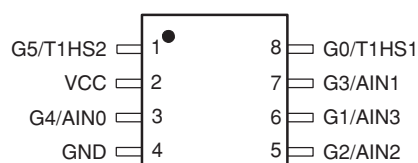
FMS7401L 8-Pin TSSOP
