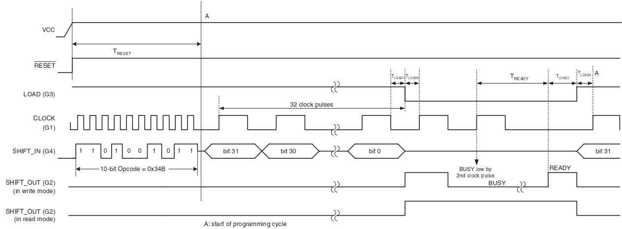
Figure 19. Programming Protocol
