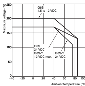
Ambient Temperature vs. Maximum Voltage (non-Latching)
