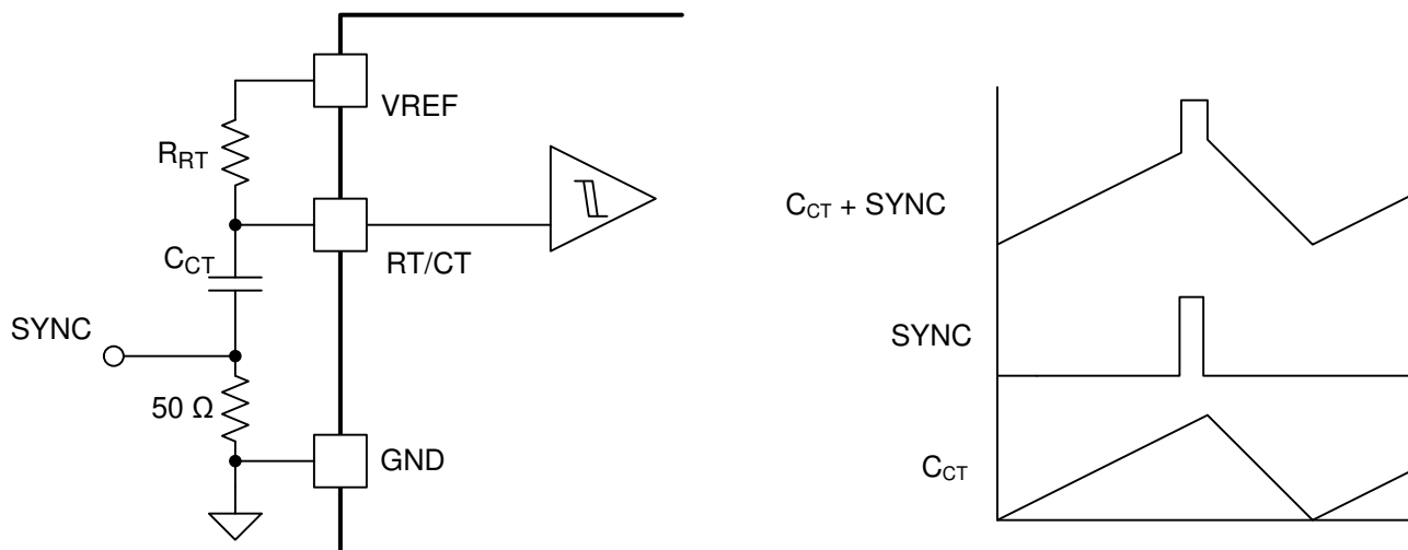
Figure 8-5. Oscillator Synchronization Circuit
