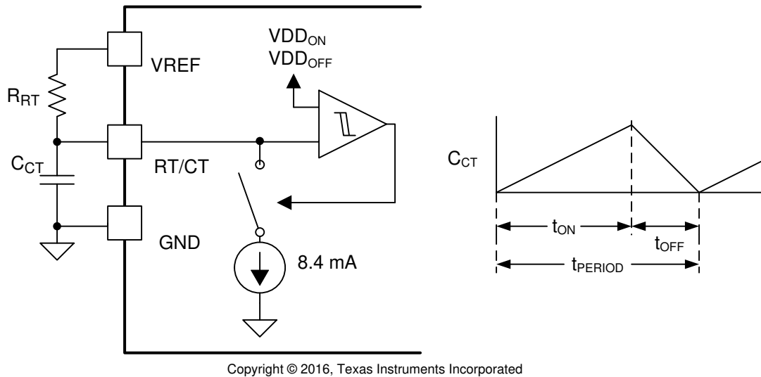
Figure 8-4. Oscillator Circuit
