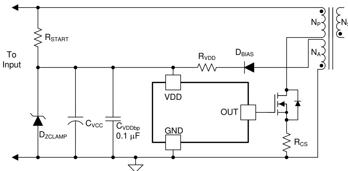
Figure 8-1. VDD Protection
