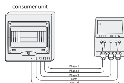
Connection schematic for three phase model
