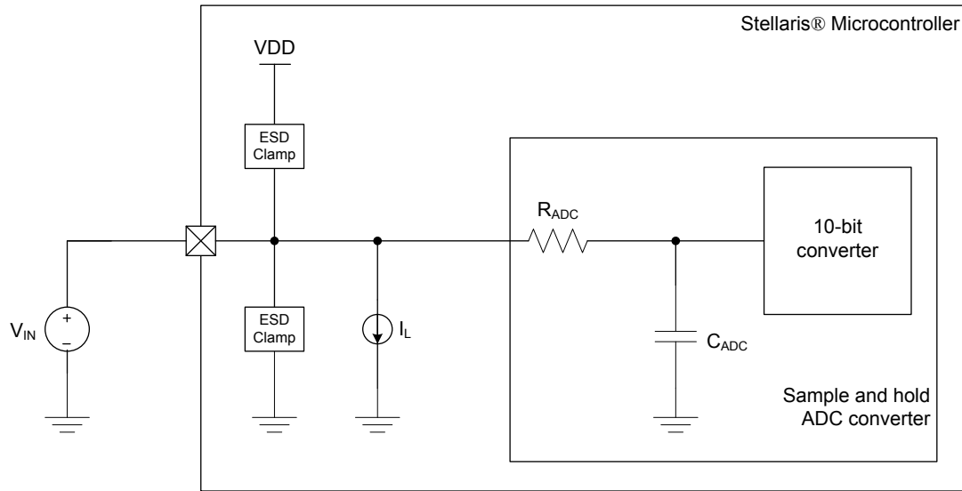
Figure 26-22. ADC Input Equivalency Diagram
