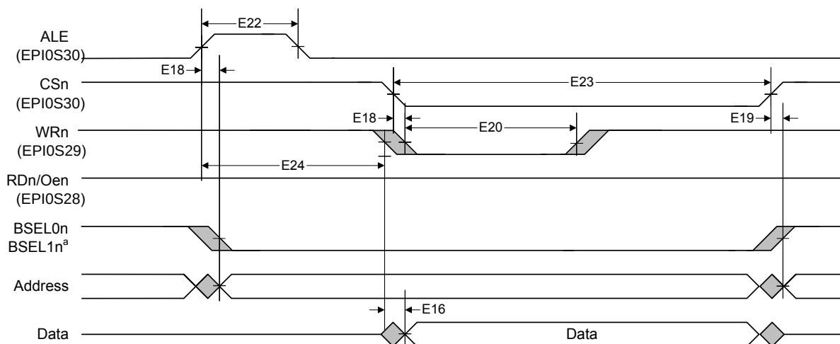
Figure 26-17. Host-Bus 8/16 Mode Write Timing
