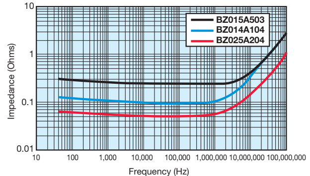
Impedance Comparison
