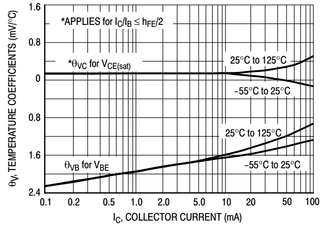
Figure 9. Temperature Coefficients
