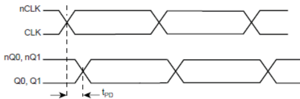
PROPAGATION DELAY
