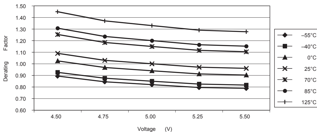
Figure 1-34 • 40MX Junction Temperature and Voltage Derating Curves (Normalized to T_J = 25^\circ\text{C} , V_{CC} = 5.0\text{ V} )
