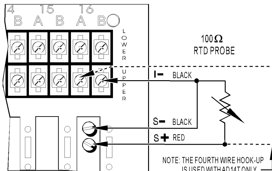
RTD CONNECTION DIAGRAM
