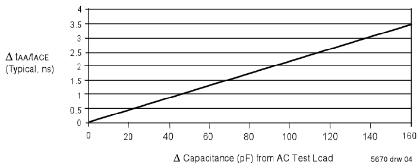
Figure 3. Typical Output Derating (Lumped Capacitive Load).
