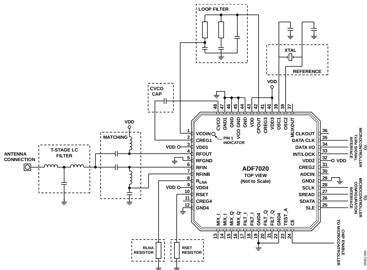
Figure 41. Application Circuit
